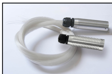
Type LED-001/W 5VDC 1W white LED or Other color on option Aluminium housing 10mm common end O 35xH115mm
