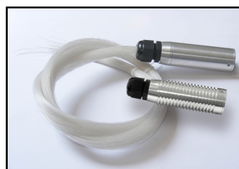
Type LED-003/3RGB 5VDC 3x1W RGB LED Aluminium housing RGB 7 colors mixing 10mm common end O 35xH130mm
