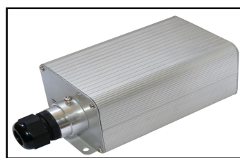
Type LED-003/MD/Al 12VDC As type LED-003/MD but Aluminium case L125xW85xH53mm
