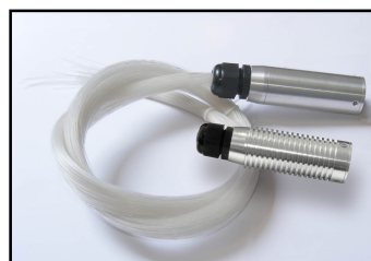
Type LED-003/W 5VDC 3W white LED or other Color on option Aluminium housing 10mm common end O 35xH115mm
